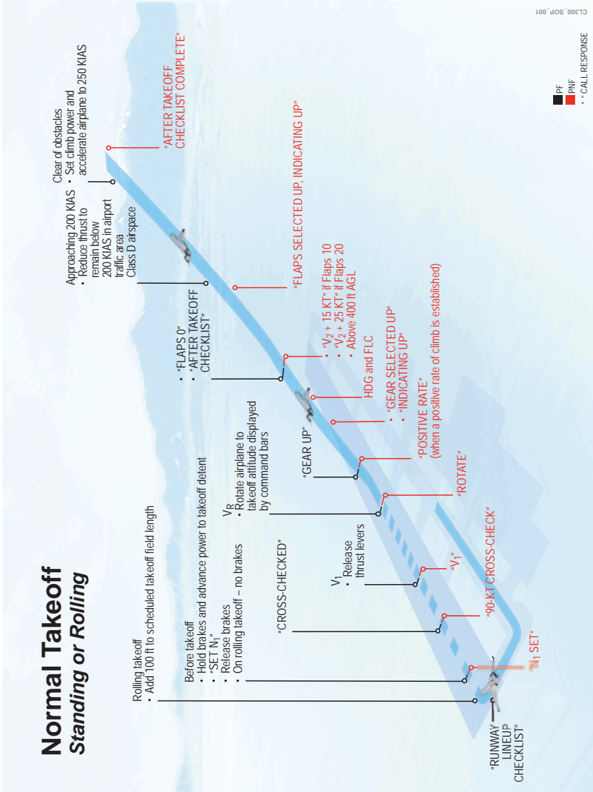
Normal Takeoff – Standing or Rolling Figure 09-12-01
